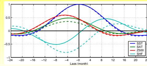
FIGURE 3: Zonal mean of time lagged crosscorrelation along 55°S for ocean forced (dashed lines) and coupled (plain lines) simulations between SST and itself (heavy blue), SAT (green), Z500 (red) and SHF (light blue).
