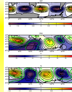
FIGURE 4: Differences between mean fields from positive and negative anomalies simulations with a 1K SSTa wavetrain of zonal mode 2 centered on 52°S. Upper SST field, lower Z500 and T500 fields. Green lines indicates 99% (plain) and 95% (dashed) significance level.
