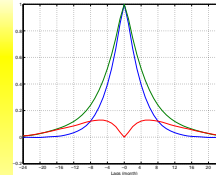
FIGURE 6: Lagged auto-correlation of SST for coupled model (green) and ocean-forced model (blue) with doubled SHF. Difference between coupled and forced ocean in red.
